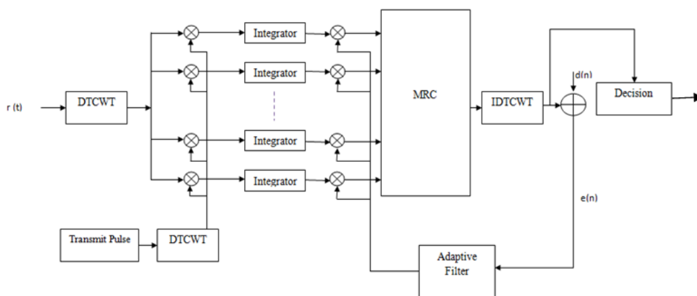
Fig.2. Proposed DTCWT Based Adaptive Rake Receiver Architecture.
